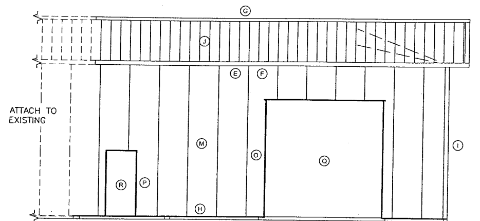
B2 SIDEWALL 1 ELEVATION 3/32" = 1'-0"
