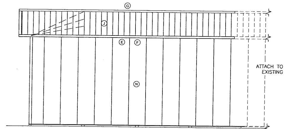
D2 SIDEWALL 2 ELEVATION 3/32" = 1'-0"
