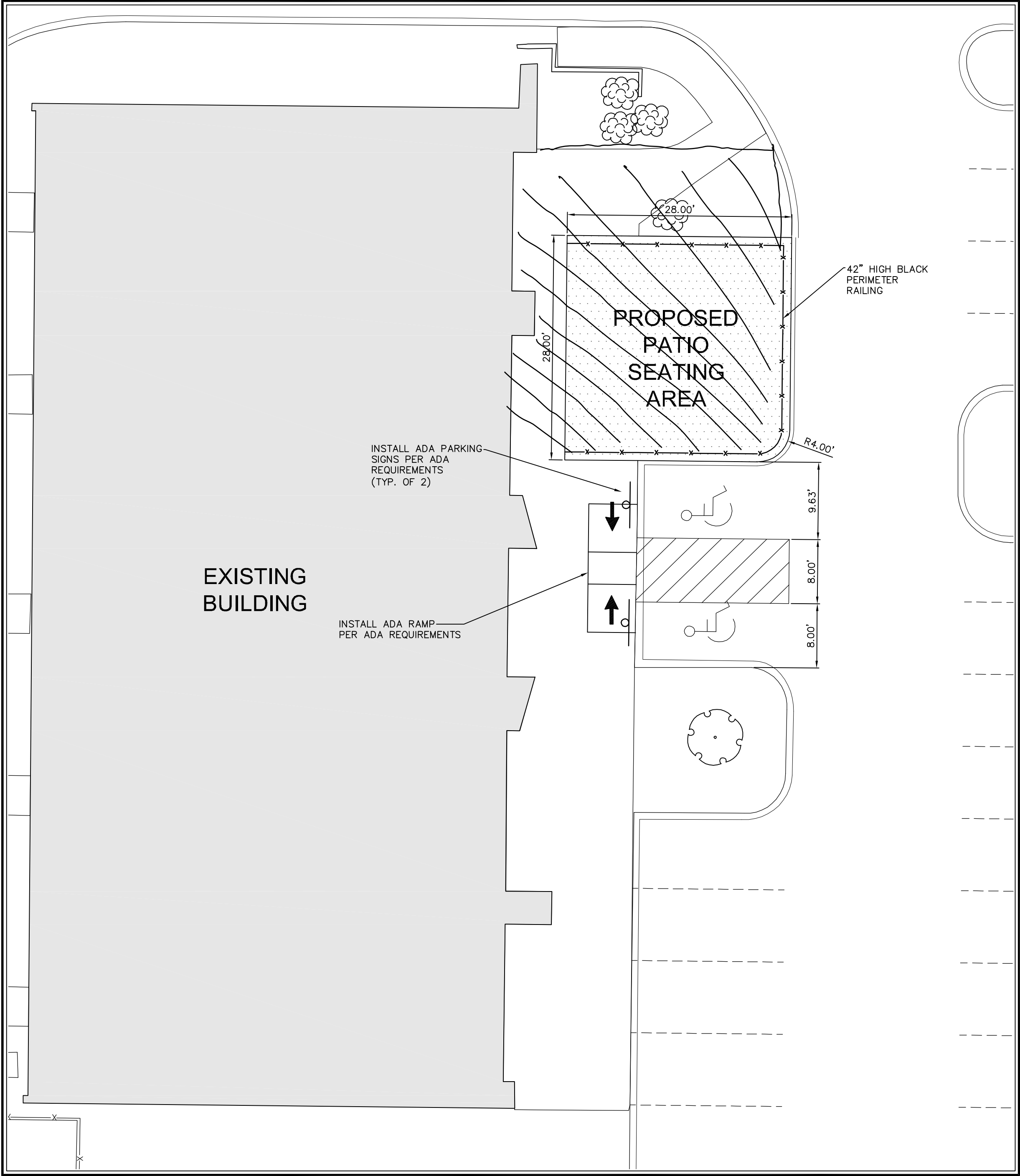
PATIO DETAIL SCALE: 1"=10'
