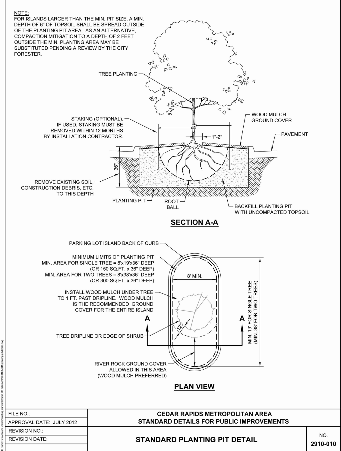
2 TYPICAL PLANTING PIT DETAIL FOR PARKING LOT ISLANDS L1.0 CITY DETAIL 2910-010
