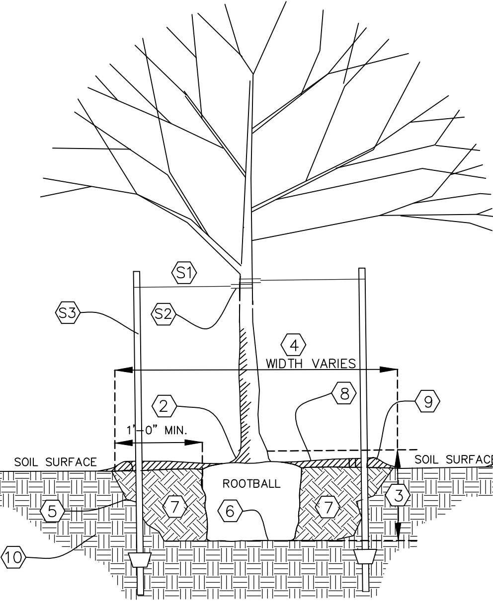
1 TREE / SHRUB / PERENNIAL INSTALLATION DETAIL L1.0 NOT TO SCALE
